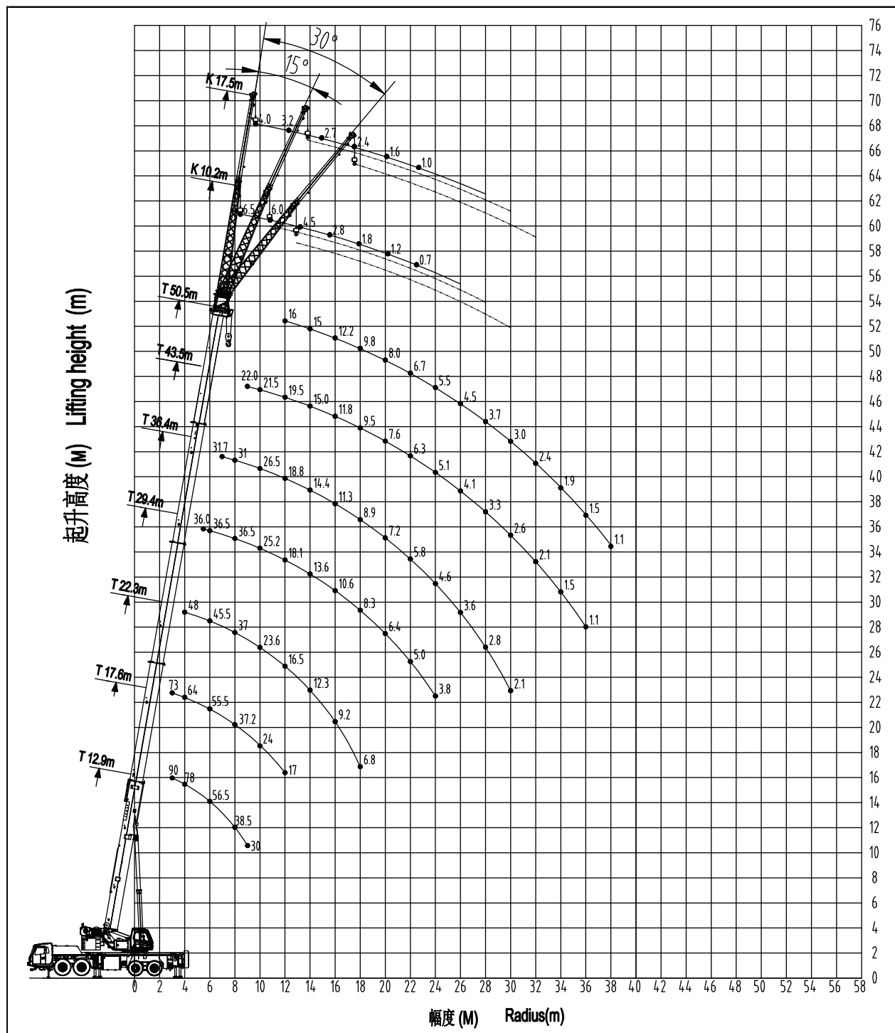
Fig2-1 Telescopic boom (T)/Telescopic boom + folding jib
