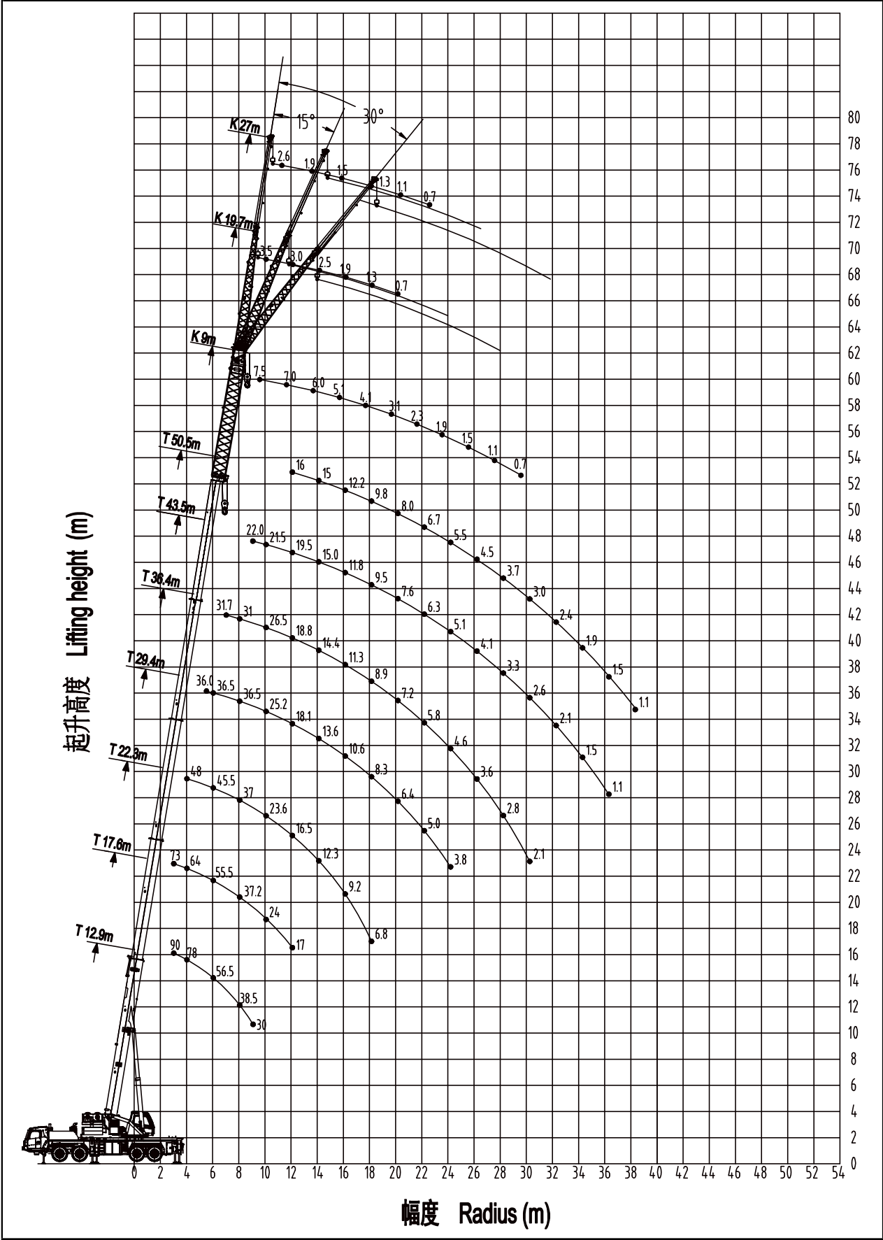
Fig2-2Telescopic boom + boom extension + folding jib (TEJ)
